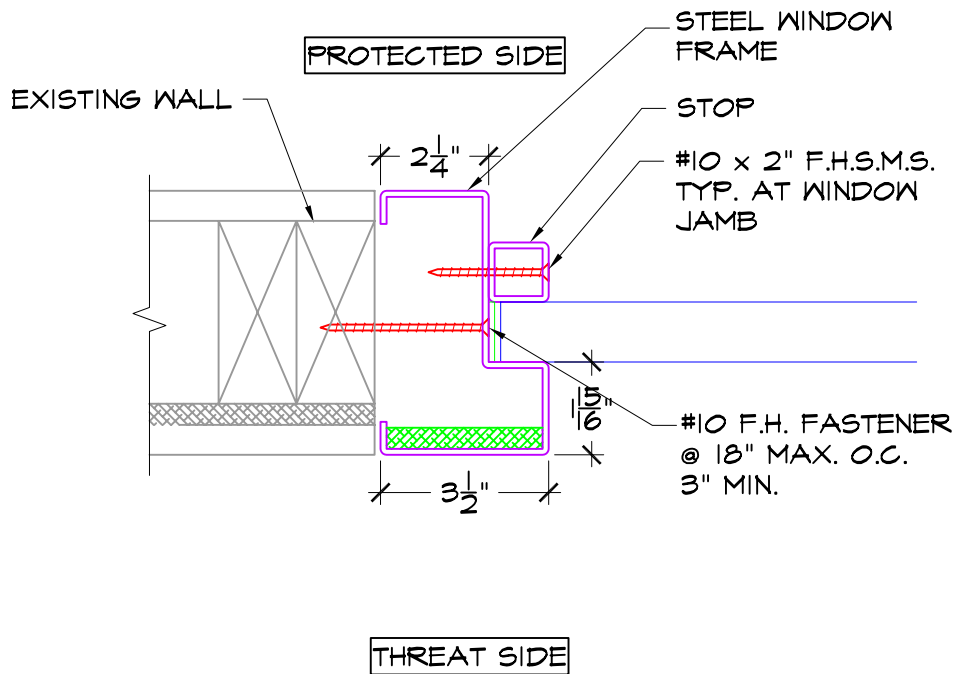
# STL. WINDOW JAMB SIM @ HEAD 3"=1'-0"
