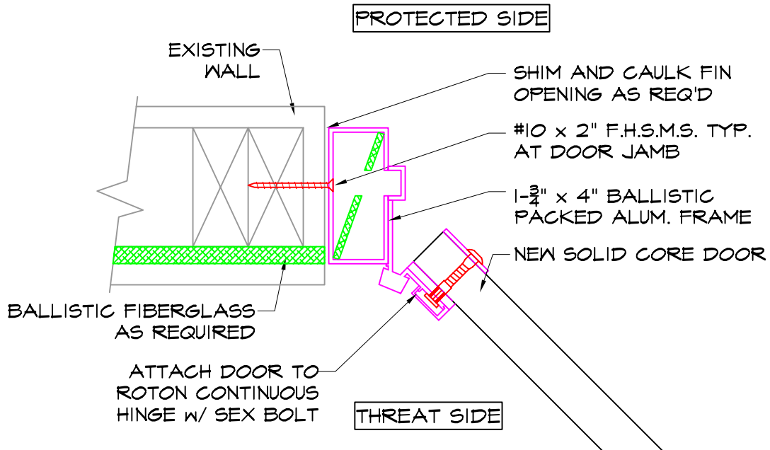
1 SOLID CORE DOOR JAMB SIM @ HEAD 3"=1'-0"
