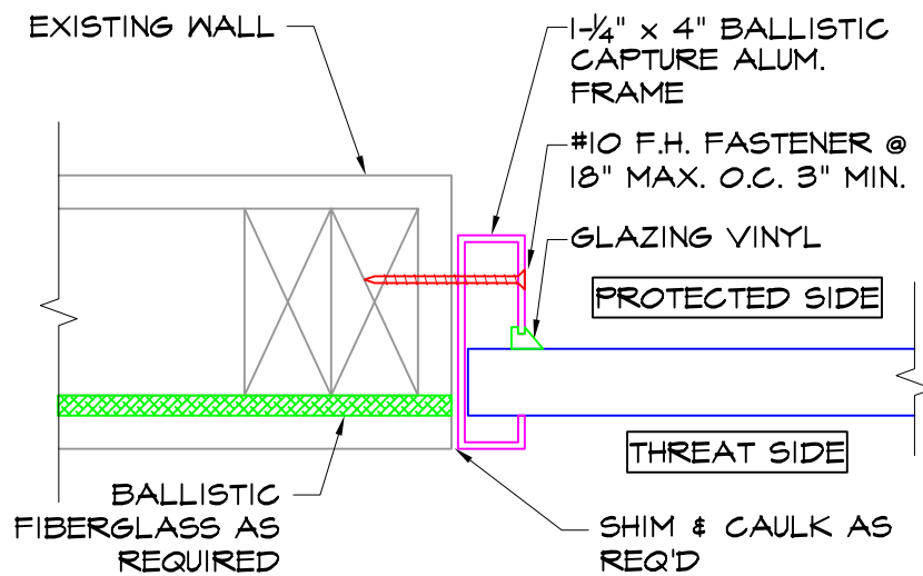
① WINDOW JAMB SIM @ HEAD 3" = 1'-0"
