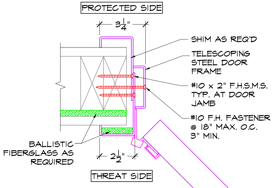
1 STL. DOOR JAMB DETAIL MADE W/10 GAUGE STEEL SIM @ HEAD 3"=1'-0"
